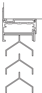
GAS-Y52 開口率=52%
